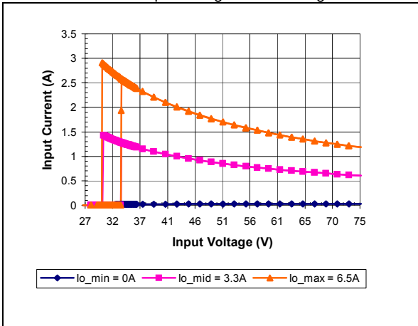
iEA48007A120V-000 Typical Input Current vs. Input Voltage Characteristics
